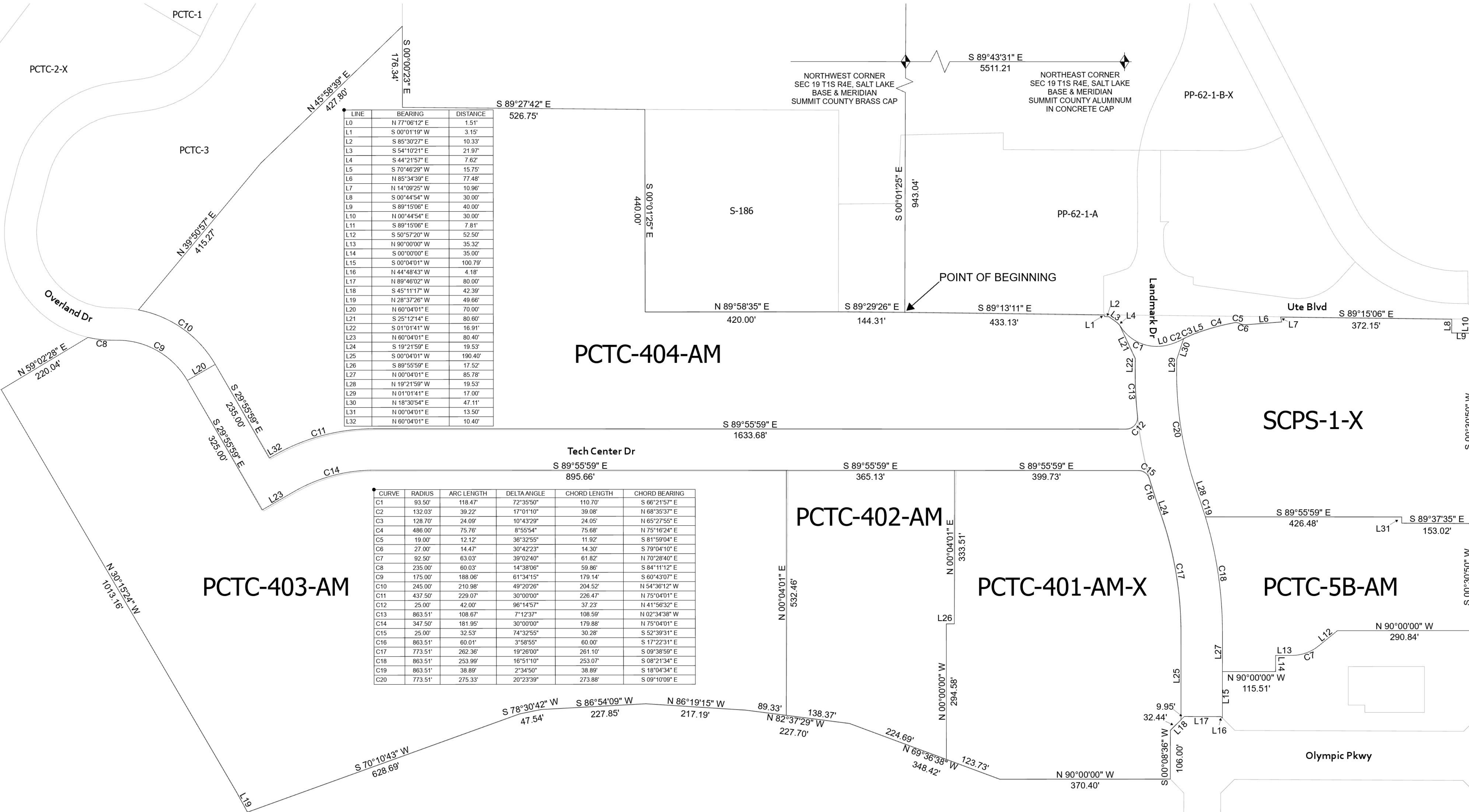
VICINITY MAP
